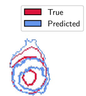
segmentations
